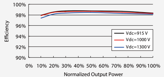
Efficiency Curve
