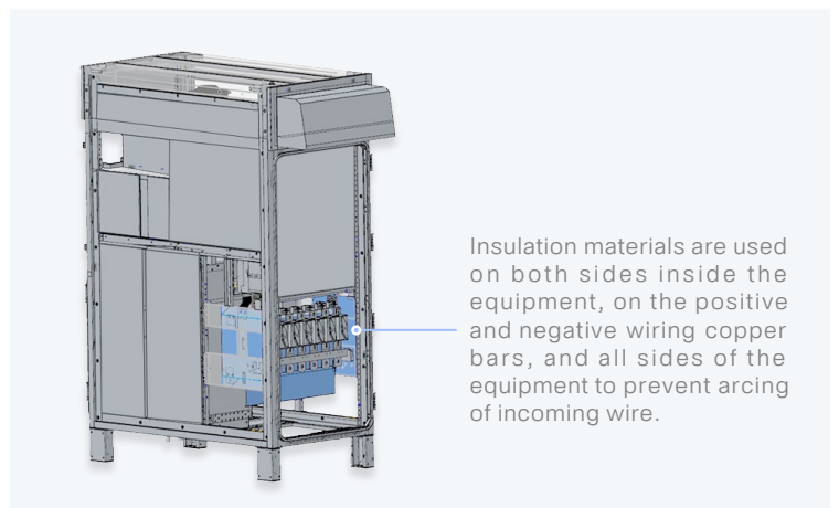
Figure 23 Design of insulation material inside equipment
