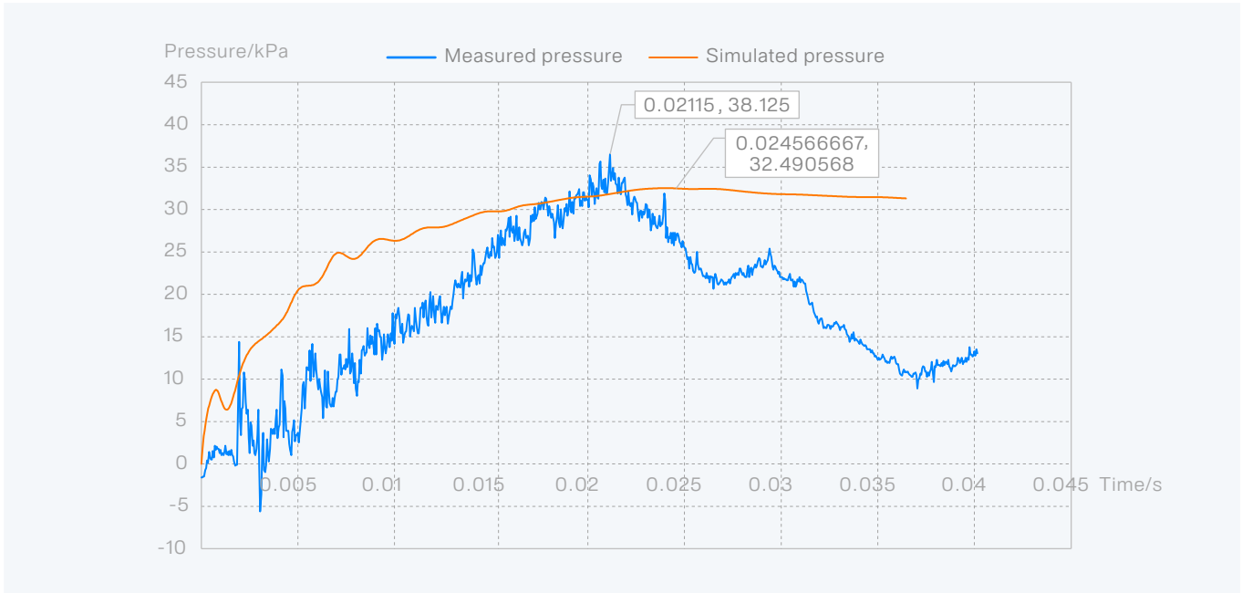
Figure 10 Comparison of simulated pressure and measured pressure
